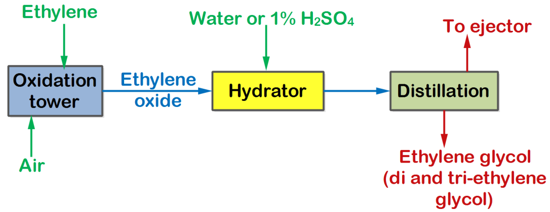
Figure: Manufacture of Ethylene glycol via ethyleneoxide
